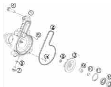
WATER PUMP
