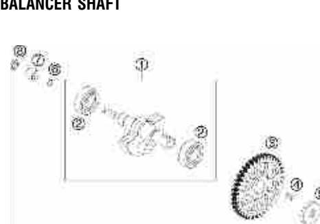
BALANCER SHAFT
